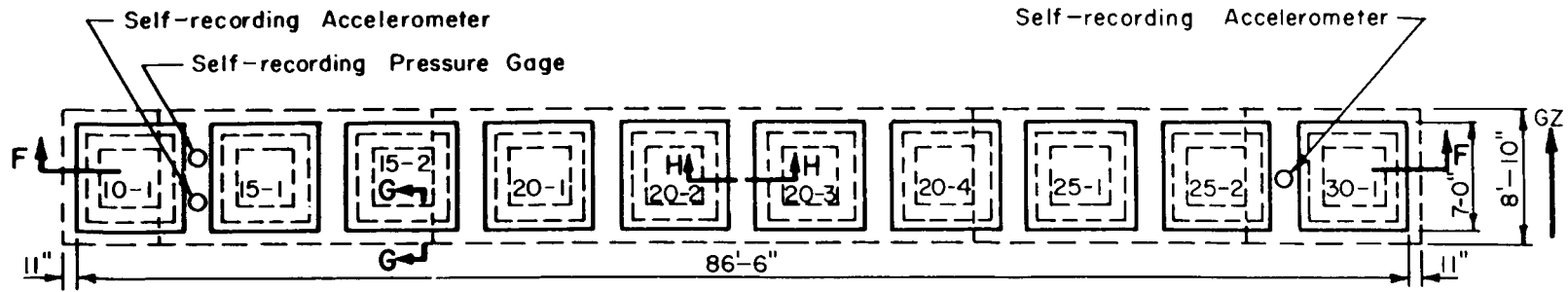
PLAN
